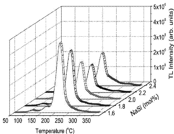
Fig. 8. The glow curves for different Na,Si concentrations. Mg: 0.2 mol% and Cu: 0.6 mol%.
