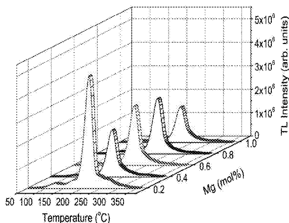
Fig. 6. The glow curves for different Mg concentrations. Cu: 0.6 mol% and Na,Si: 2.0 mol%.
