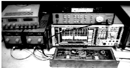
Fig. 6. Microwave power amplifier setup of measurement.
