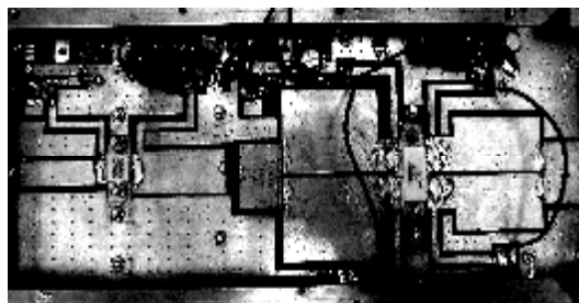
Fig. 5. Microwave power amplifier. First stage of 45W, second stage of 90W of an input 300mW.
