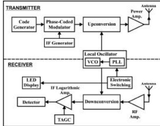
Fig. 1. Block diagram of typical radar system.
