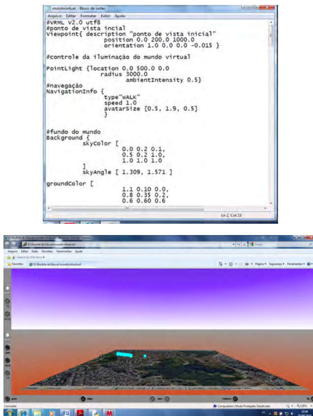
Fig. 2. VRML textual code and its symbolic representation using the concept of metadata in (Pocsa et al., 1998) and supporting individuals' tacit knowledge, digital literacy skills and cognition improvements such as attention, planning, critical thinking and memory through programming, saving and debugging the VRML file as well as enhancing ones' writing, reading and visualization abilities and competences.
