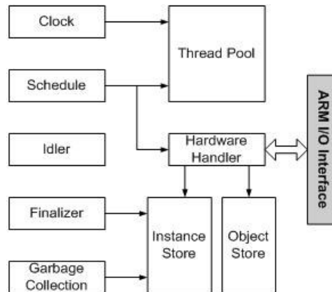
Figure 5. Kaffe design of co-processor.
