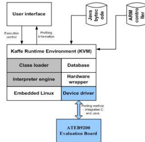
Figure 3. Integrated platform.
