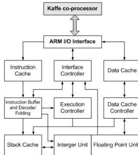
Figure 4. Hardware design based on an ARM processor.
