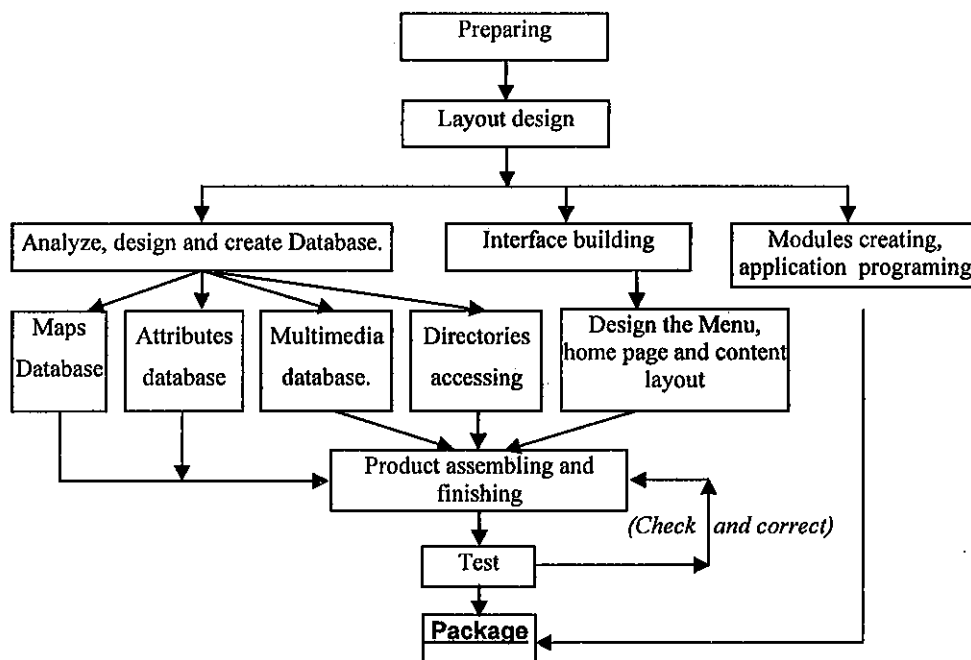
Fig. 1. Building Diagram of Atlas.
