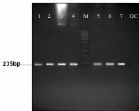
Fig 2. Electrophoresis of PCR products OPRM1 gene on agarose 1.5%, 60V. DC: negative control; lane 1-7: PCR products; M: DNA marker 1kb.
