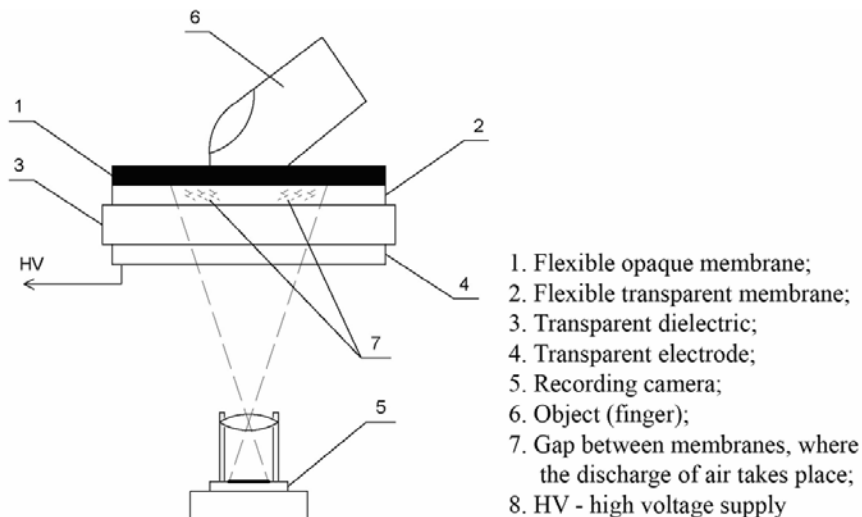
Fig. 2. Schema of the BHT-capturing module
