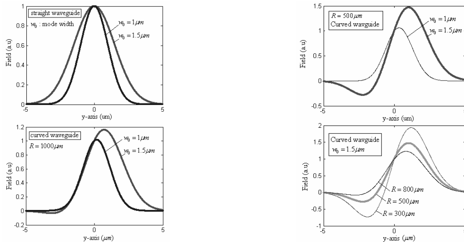
Fig. 3. Field profiles for a straight waveguide and a bent waveguide at different radii.
