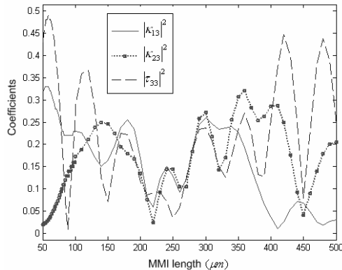
Fig. 8. Matrix coefficients of the higher order mode at input port 2 coupled to output ports.
