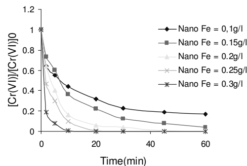
Fig. 4. Effect of iron nanoparticles concentration.
