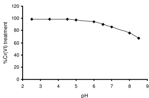
Fig. 2. Effect of the initial pH value on the rate of Cr(VI) reduction.
