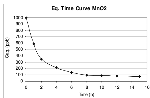
Fig. 4. Reduction of arsenic concentration upon the sorption time.
