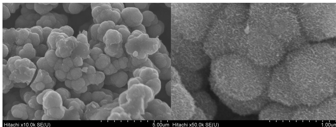
Fig. 3. SEM image of denaturated laterite surface after nano \text{MnO}_2 coating.
