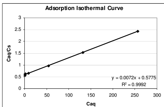
Fig. 5. The Langmuir adsorption Isothermal Curve.
