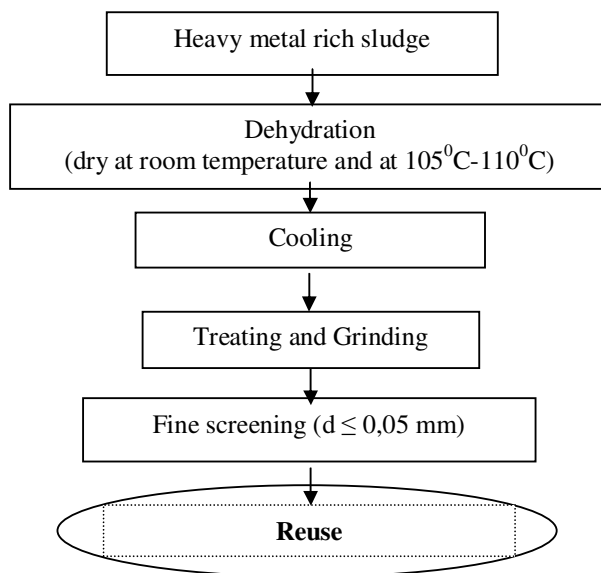
Fig. 1. Diagram of thickened sludge treatment.
