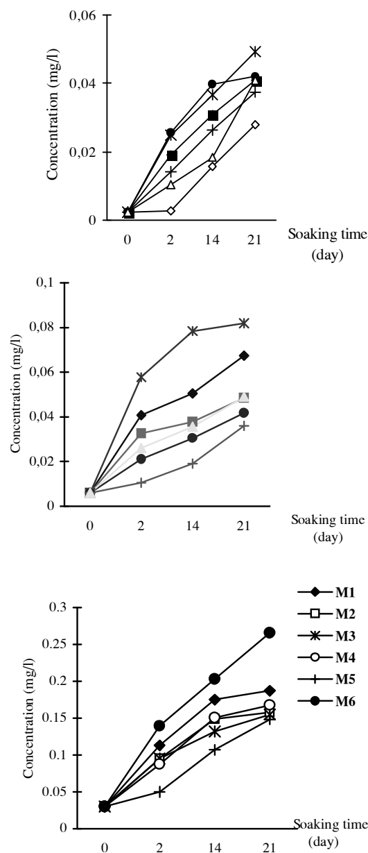
Fig. 2. Concentration of some heavy metals existing in sludge in the rain water soaking with bricks:
