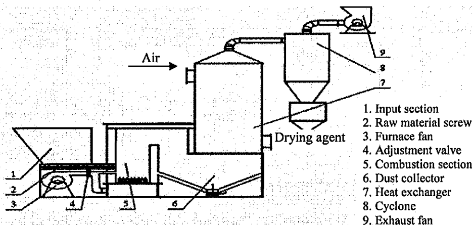
Fig. 2. The scheme of structure of FBC.
