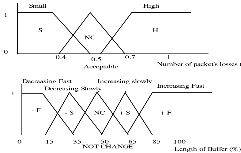
Figure 4. Membership functions for input variables.
