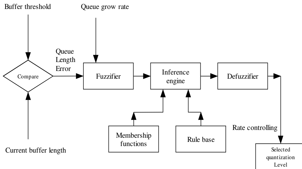
Figure 3. Block diagram of fuzzy control system.
