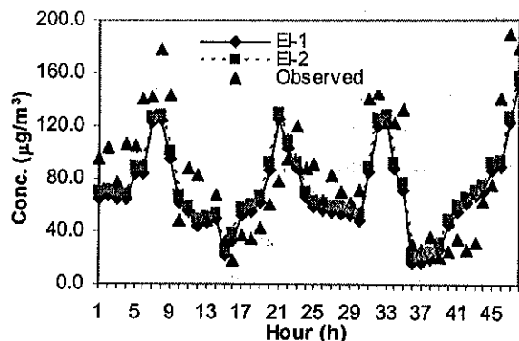
Fig. 1. Comparison CO conc. at HB station (left) and NO x conc. at BC station (right) on Jan. 19&20, 2006.
