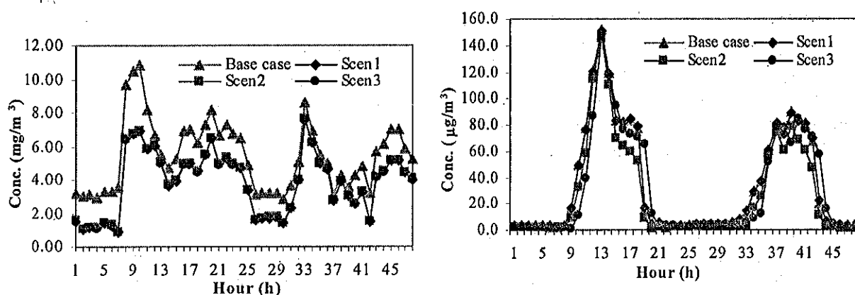
Fig. 8. Comparison CO conc. at HB station (left) and Ozone conc. at DO station on Jan. 19&20, 2006.
