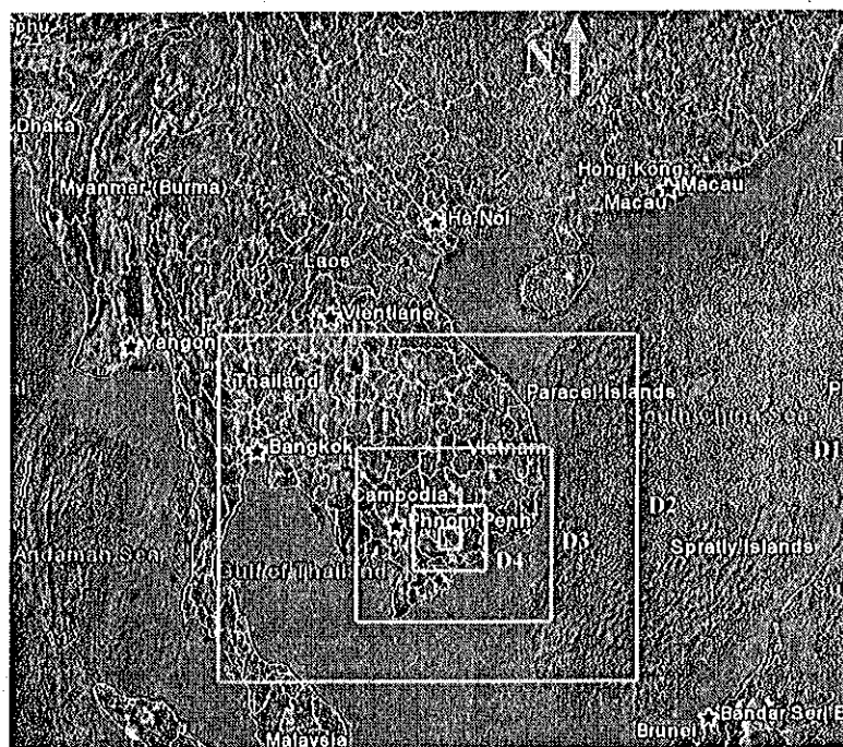
Fig. 4. Domains for meteorological simulation.
