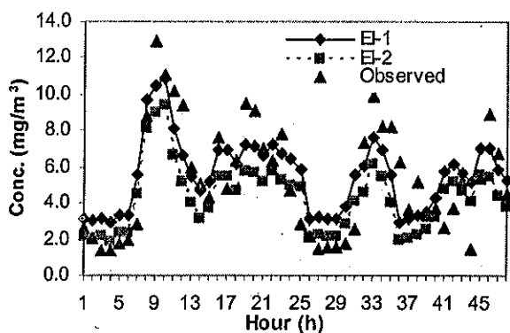
Fig. 1. Comparison CO conc. at HB station (left) and NO x conc. at BC station (right) on Jan. 19&20, 2006.
