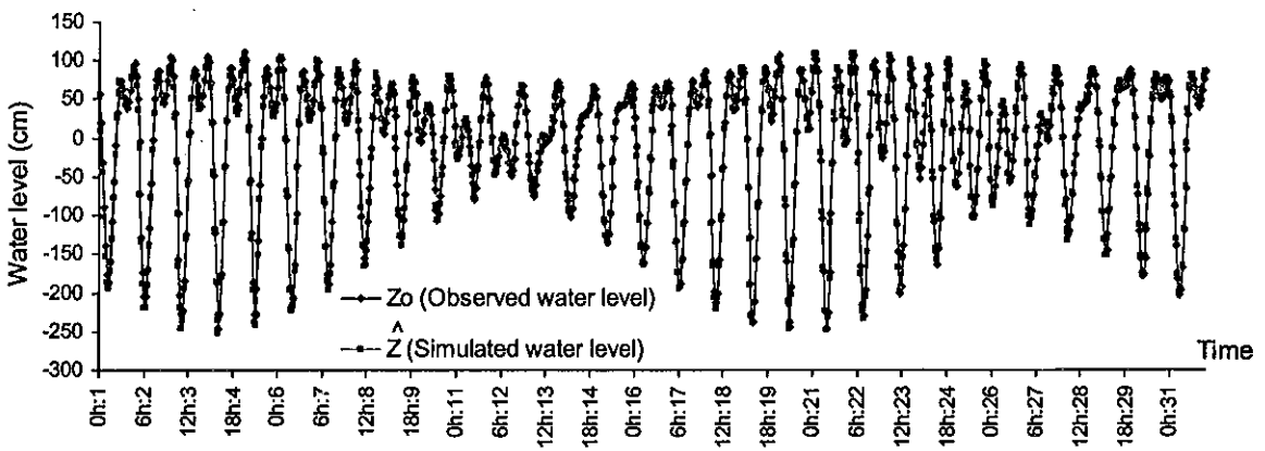
Fig. 4. The observed and simulated water level in Jan/2007 of Vung Tau station.
