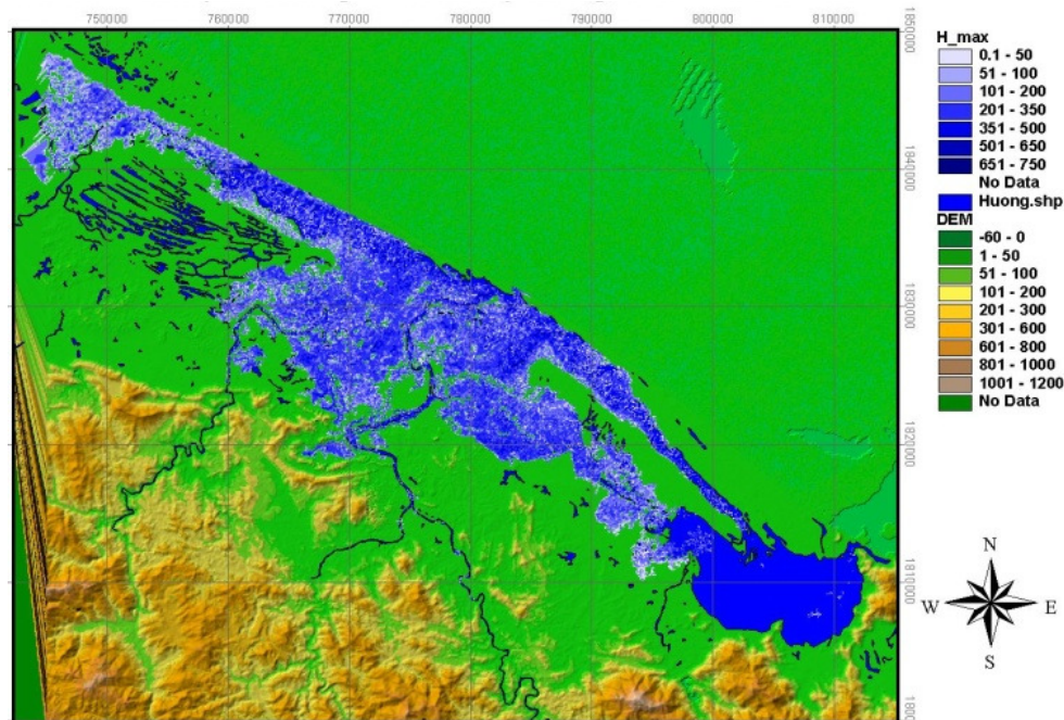
Figure 2. Inundation map for the year 2100 under B2 scenario.
